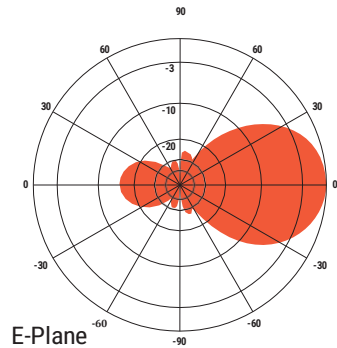
ANT740Y8-WR at 740 MHz
