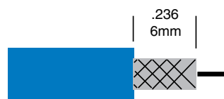
TWO STEP (2 BLADES) RFA-4086-006
