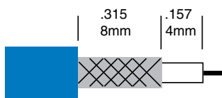
THREE STEP (3 BLADES) RFA-4086-003
