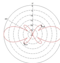
E-Plane Pattern
