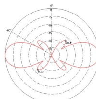
E-Plane Pattern
