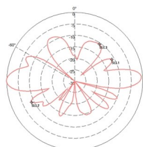
E-Plane Pattern
