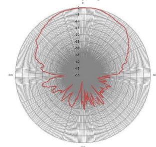
E Plane
